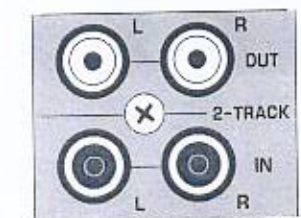
Fig. 2.11: 2-Track Input/Output
